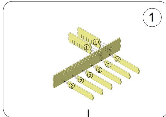
Main box assembly
