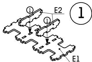
Assistant tray (Parts E; Sheet 8)
