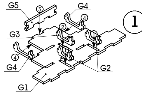
Temple tiles tray (Parts G; Sheet 8)
