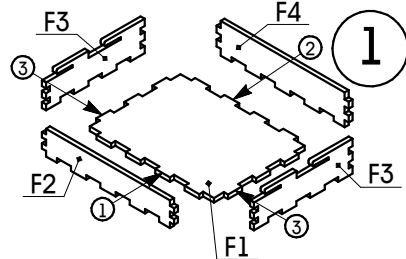
Player tray (x4) (Parts F; Sheets 9, 10)
