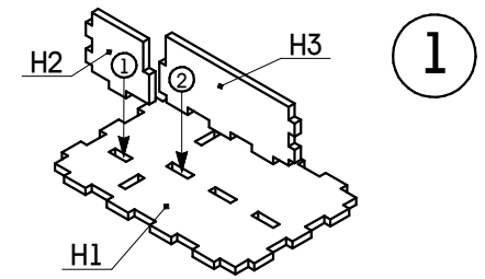
Tiles tray (Parts H; Sheet 7)
